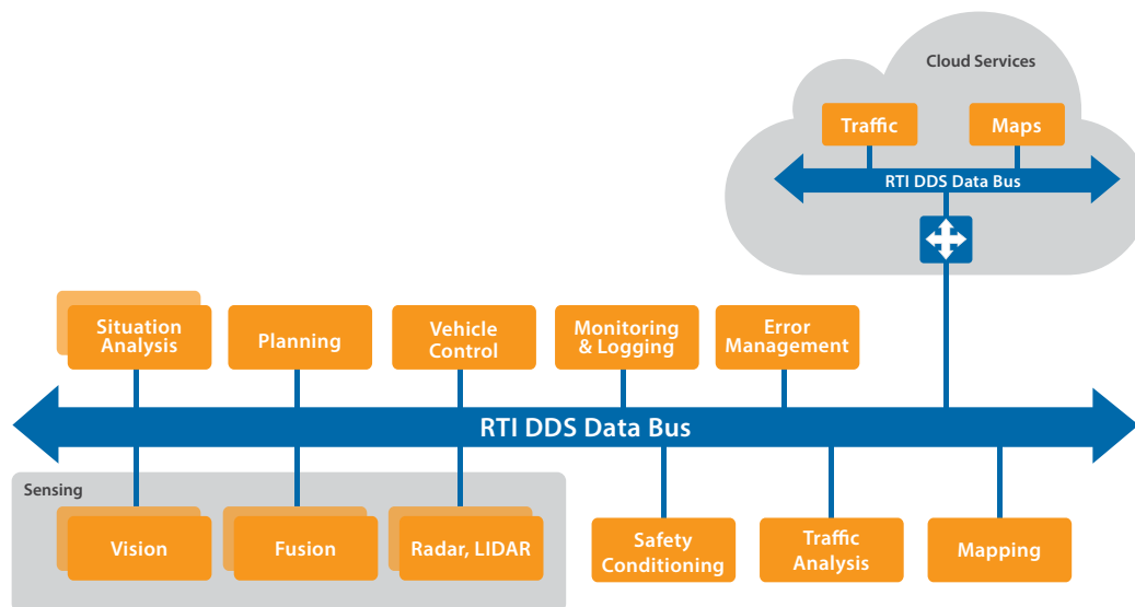
Figure 3. DDS in Connected Vehicle Architecture
