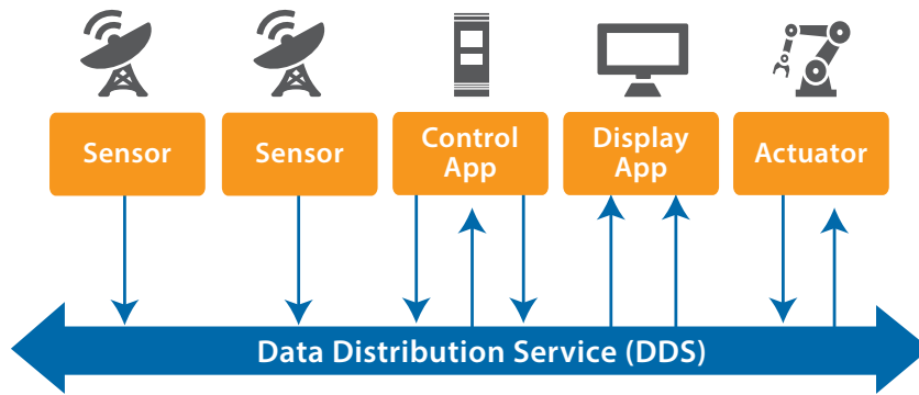
Figure 2. DDS enables seamless connectivity between sensors, actuators and applications
