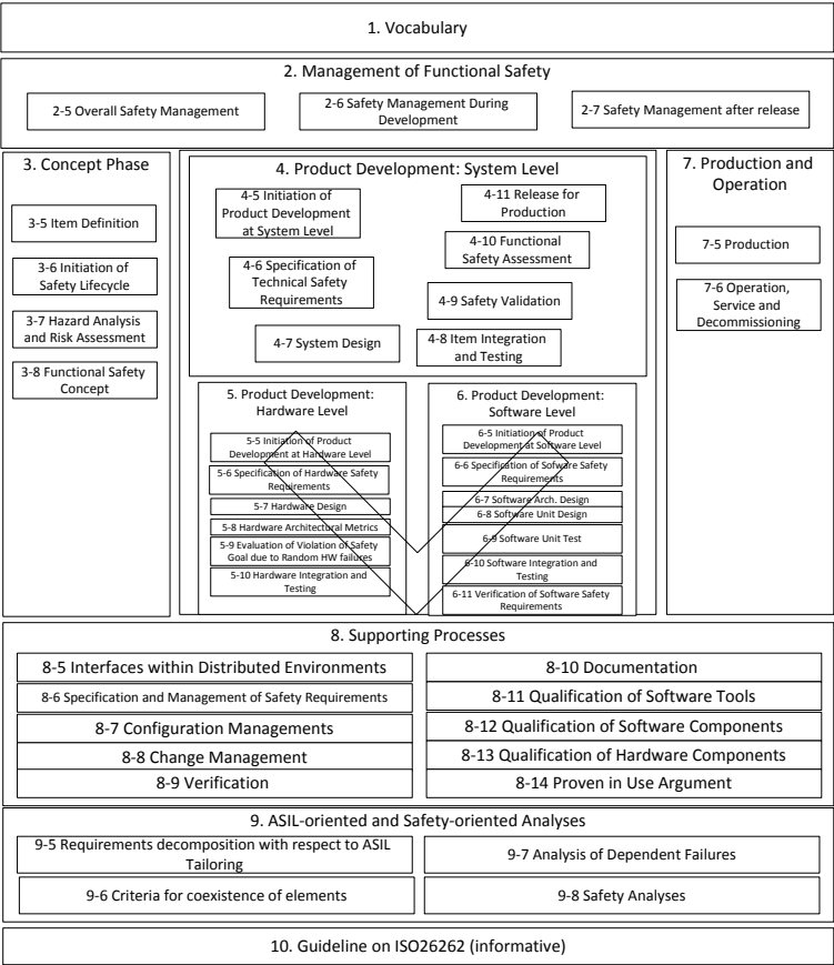
Figure 1: ISO 26262 Processes and Requirements (ref. ISO 26262)
