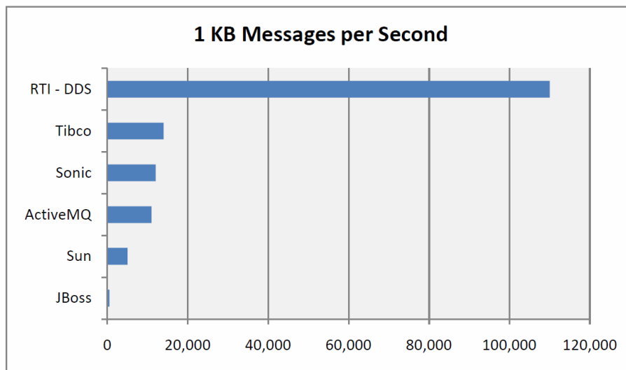
Figure 2: JMS performance of RTI Data Distribution Service vs. other message-centric middleware
