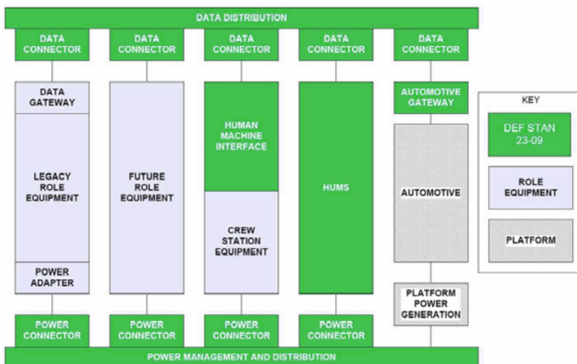
Figure 1: GVA Def Stan 23-09 architectural overview
