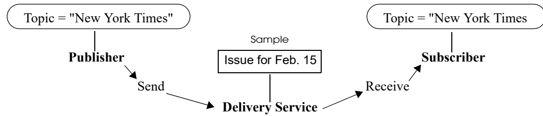
Figure 2.1 Publish-Subscribe Example
